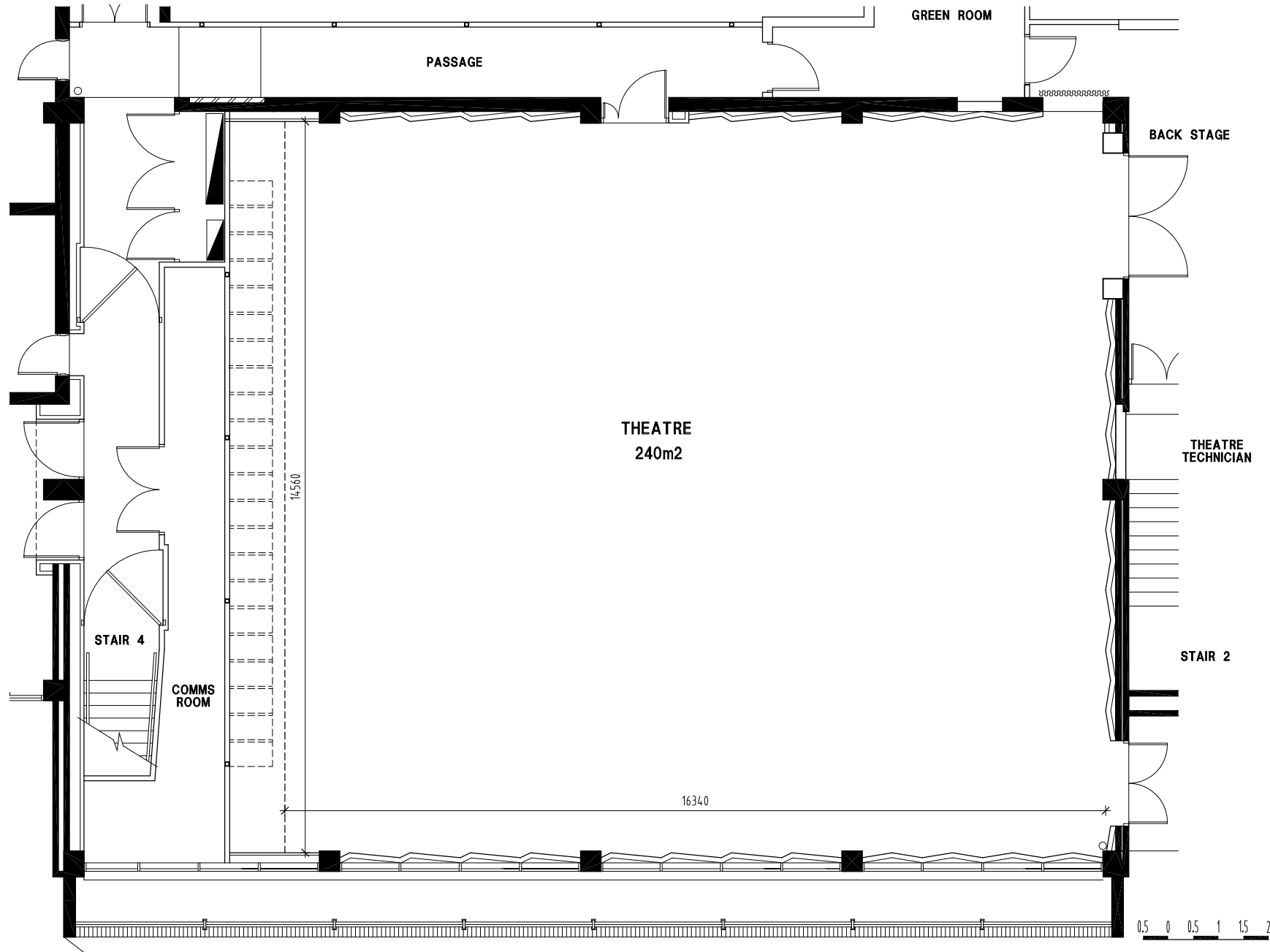
Theatre Plan
